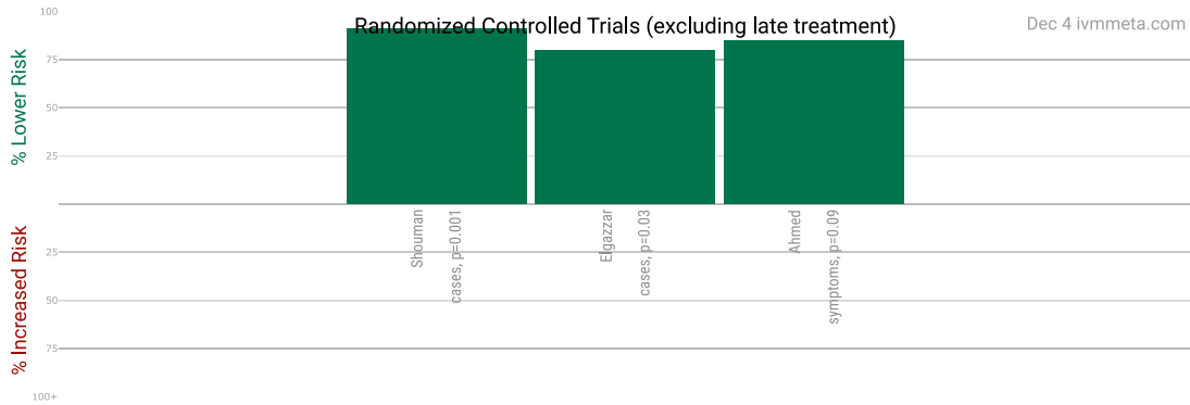
Figure 8. RCTs excluding late treatment.
