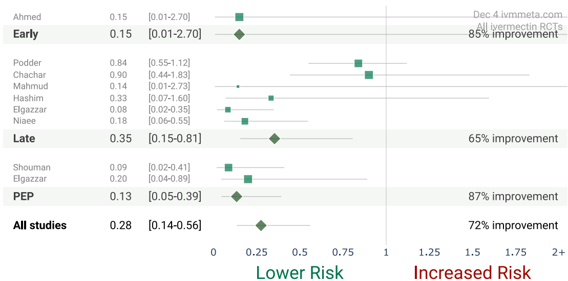
Figure 9. Forest plot (random effects model) for Randomized Controlled Trials only.
