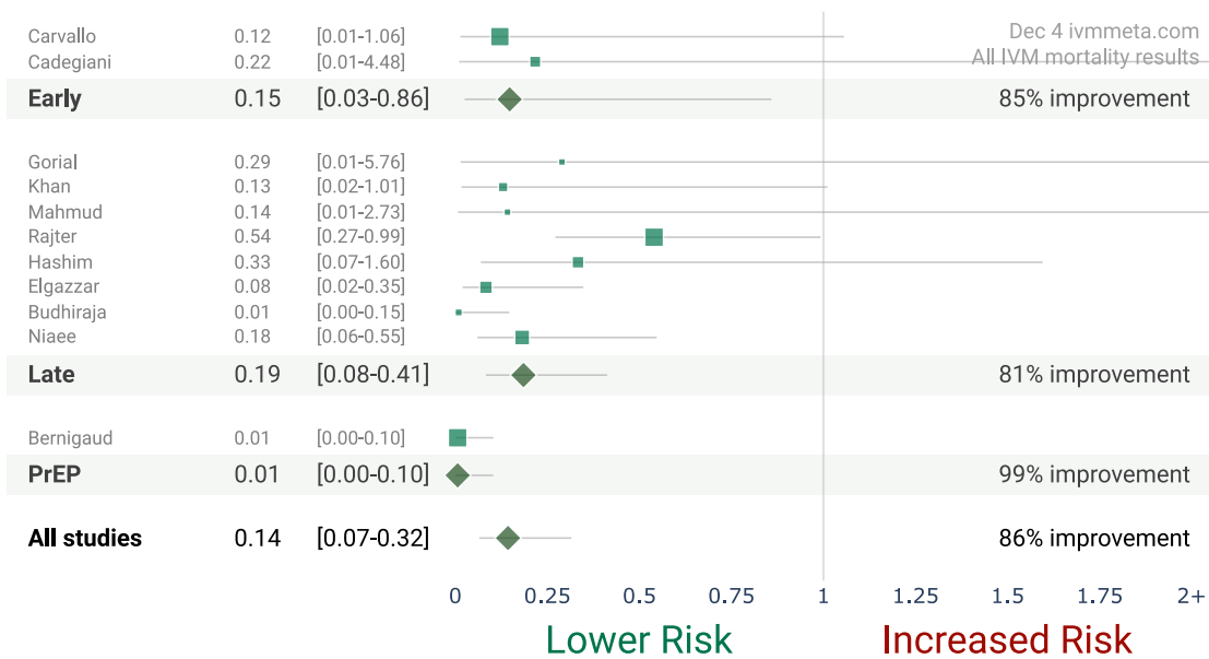
Figure 6. Forest plot (random effects model) for mortality results only.
