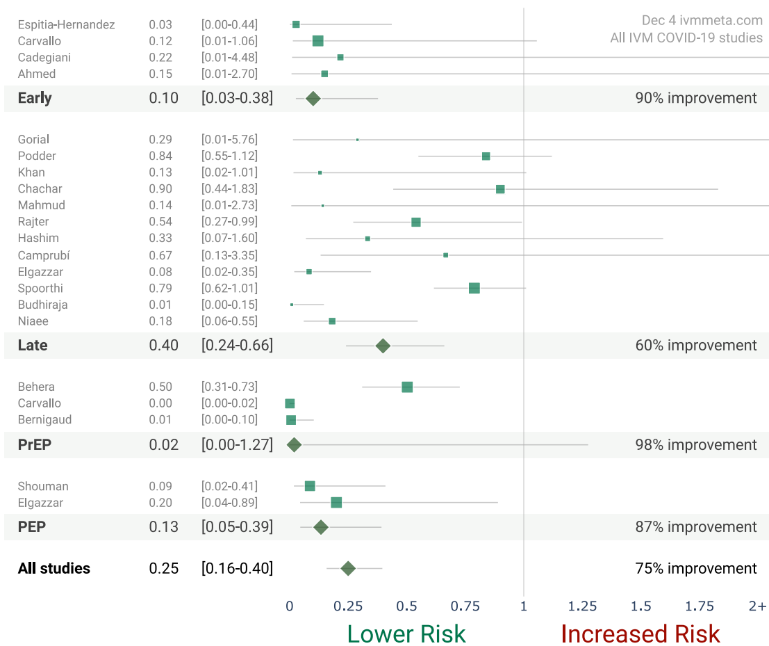
Figure 5. Forest plot (random effects model).
